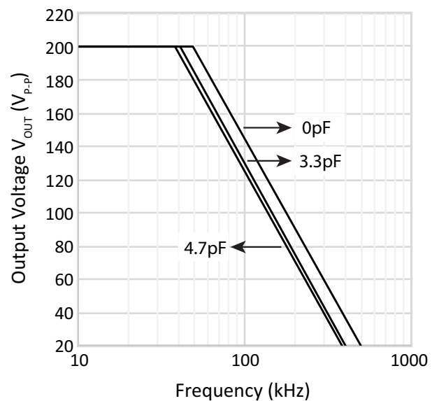
Figure 5: Power Response vs Compensation
